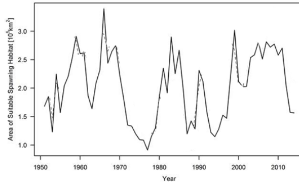
Figure 1. Time-series of the area ( \text{km}^2 ) of suitable spawning habitat of blue whiting in the month of peak larval presence (April).
