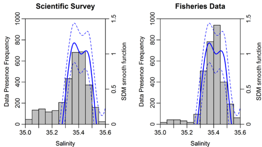
Figure 5. Presence frequency of spawning blue whiting (number of pixels with presences) observed in scientific surveys a) and caught in fisheries b) compared to the salinity (300-600 m) at which these observations were made (bars). The blue line indicates the modelled smooth function of blue whiting larval-presence obtained from the Species Distribution Model (SDM) based on larval blue whiting catches by the CPR survey d), with dashed lines indicating the standard error. Panel a) shows observations from late March/ early April, and Panel b) data shows data from March. The SDM was calibrated with CPR data from February to June.
